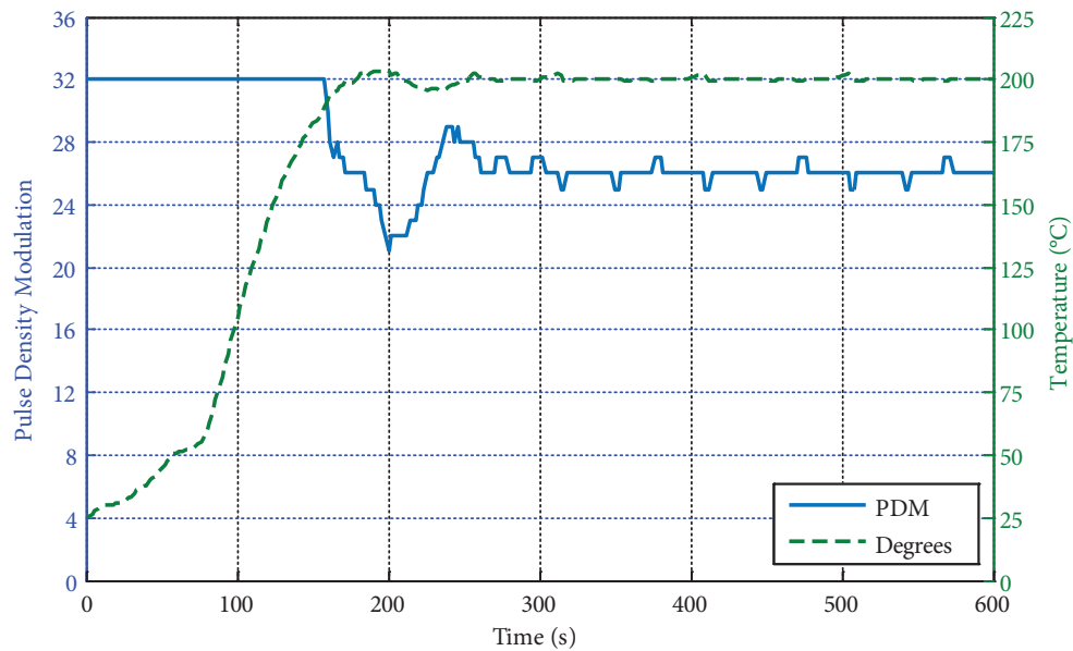
Figure 15. The PDM-temperature-time variation of the work piece.
