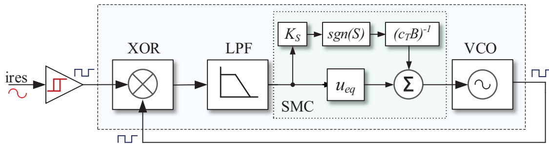
Figure 5. The block diagram of sliding-mode-controlled PLL function.
